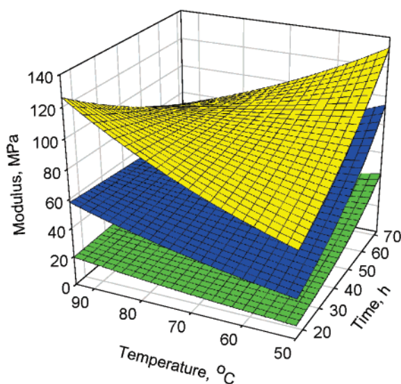
Figure 8. Response surface models for modulus graphed vs (a) APTES and epoxy concentration with time and temperature held constant at the predicted optimum values for stress, and (b) time and temperature with epoxy and APTES concentration held constant at the predicted optimum values for stress.
