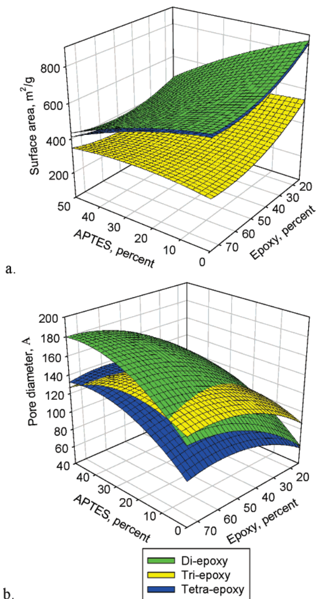
Figure 5. Response surface models for (a) BET surface area and (b) pore diameter graphed vs APTES and epoxy concentration with time and temperature held constant at the predicted optimum values for stress.
