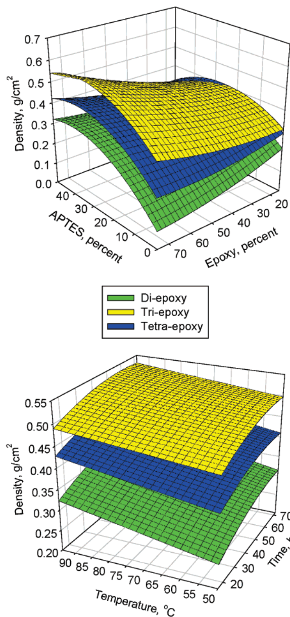
Figure 4. Response surface models for density graphed versus (a) APTES and epoxy concentration with time and temperature held constant at the predicted optimum values for stress, and (b) time and temperature with epoxy and APTES concentration held constant at the predicted optimum values for stress.
