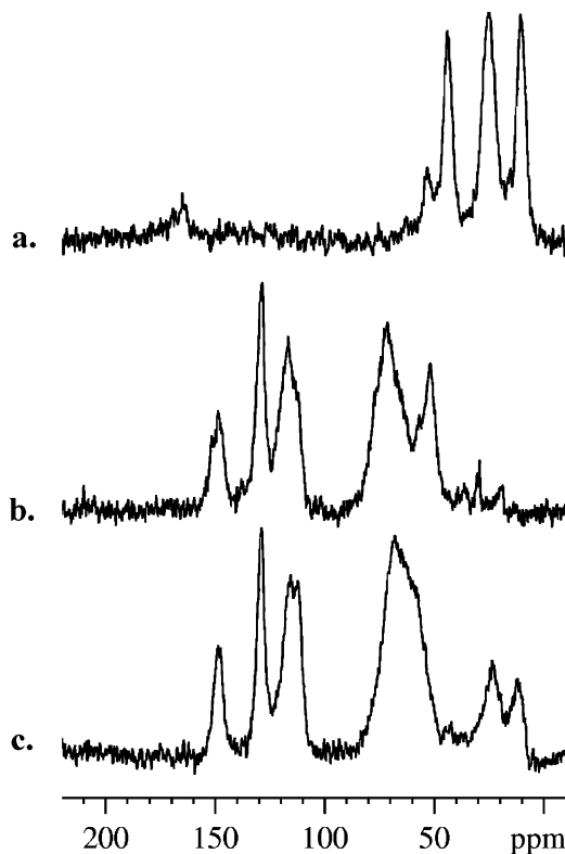
Figure 10. ^{13}\text{C} NMR of (a) 50% APTES, (b) no APTES with di-epoxy (run 21), and (c) 50% APTES with di-epoxy (run 9).
