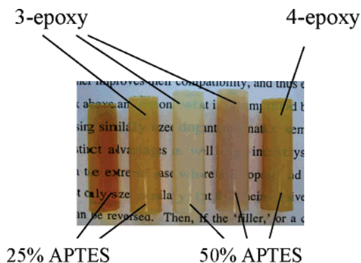
Figure 1. Photograph of representative samples of APTES-modified, epoxy cross-linked aerogels.
