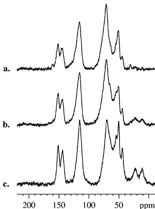
Figure 12. ^{13}\text{C} NMR of (a) no APTES with tri-epoxy (run 12), (b) 25% APTES with tri-epoxy (run 27), and (c) 50% APTES with tri-epoxy (run 20).
