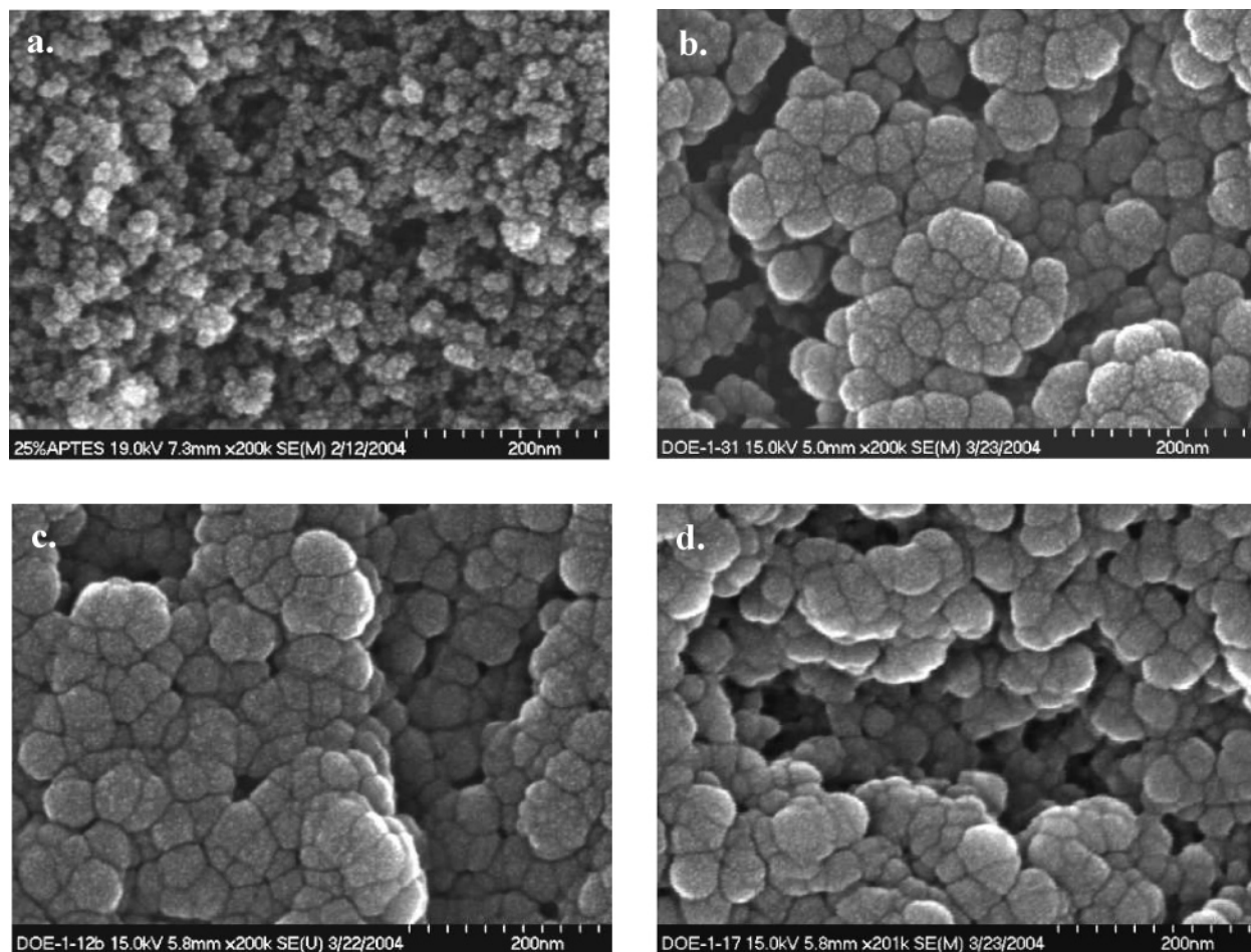
Figure 2. Scanning electron microscopy of (a) 25% APTES without epoxy, (b) 25% APTES with di-epoxy (run 30), (c) 25% APTES with tri-epoxy (run 11), and (d) 25% APTES with tetra-epoxy (run 16).
