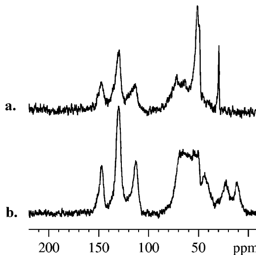
Figure 11. ^{13}C NMR of (a) no APTES with tetra-epoxy (run 3) and (b) 50% APTES with tetra-epoxy (run 19).
