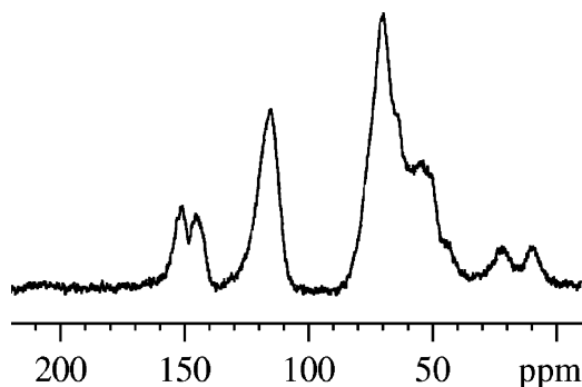
Figure 13. ^{13}\text{C} NMR of sample from run 27 (25% APTES with tri-epoxy) after 5 h post-cure at 150 °C.
